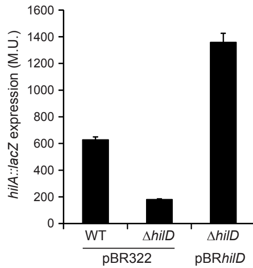
S4 Figure. The \Delta hilD - cm R mutant strain is trans-complemented by a pBR322-based plasmid carrying the hilD gene. Cultures of the strains SV5015UB2 and TGC-10 were grown in LB at 37°C up to an OD 600nm of 2.0. Data are the average and error bars represent standard deviations from three biological replicates.
