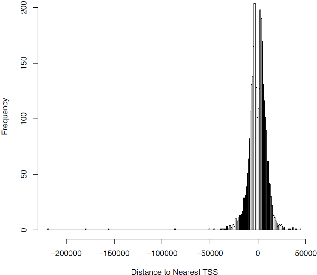
Figure S3. GCN5b distribution around transcription start sites (TSS). The distance between each GCN5b-associating site (FDR < 0.05) and the nearest TSS (based on data in Yamagishi et al. 2010) was calculated and plotted as a histogram.
