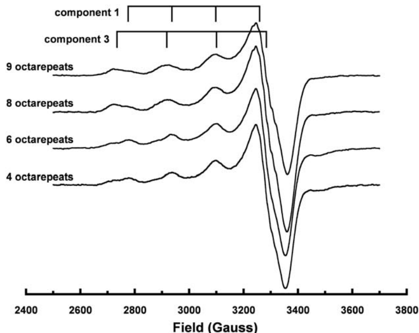
Figure 2. EPR spectra of octarepeat constructs in equilibrium with 3.0 equivalents of Cu 2+ . With four and six octarepeats, the spectra are nearly equivalent and show a mixture of component 1 and component 3 coordination. For longer octarepeat domains, there is a progressive shift to favor component 3 coordination.
