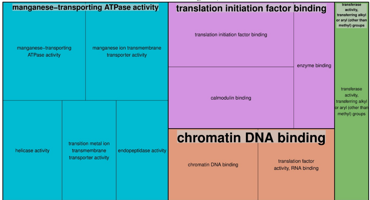
Supplementary Figure 12. Enriched GO term tree map of molecular functions for short term freezing.
