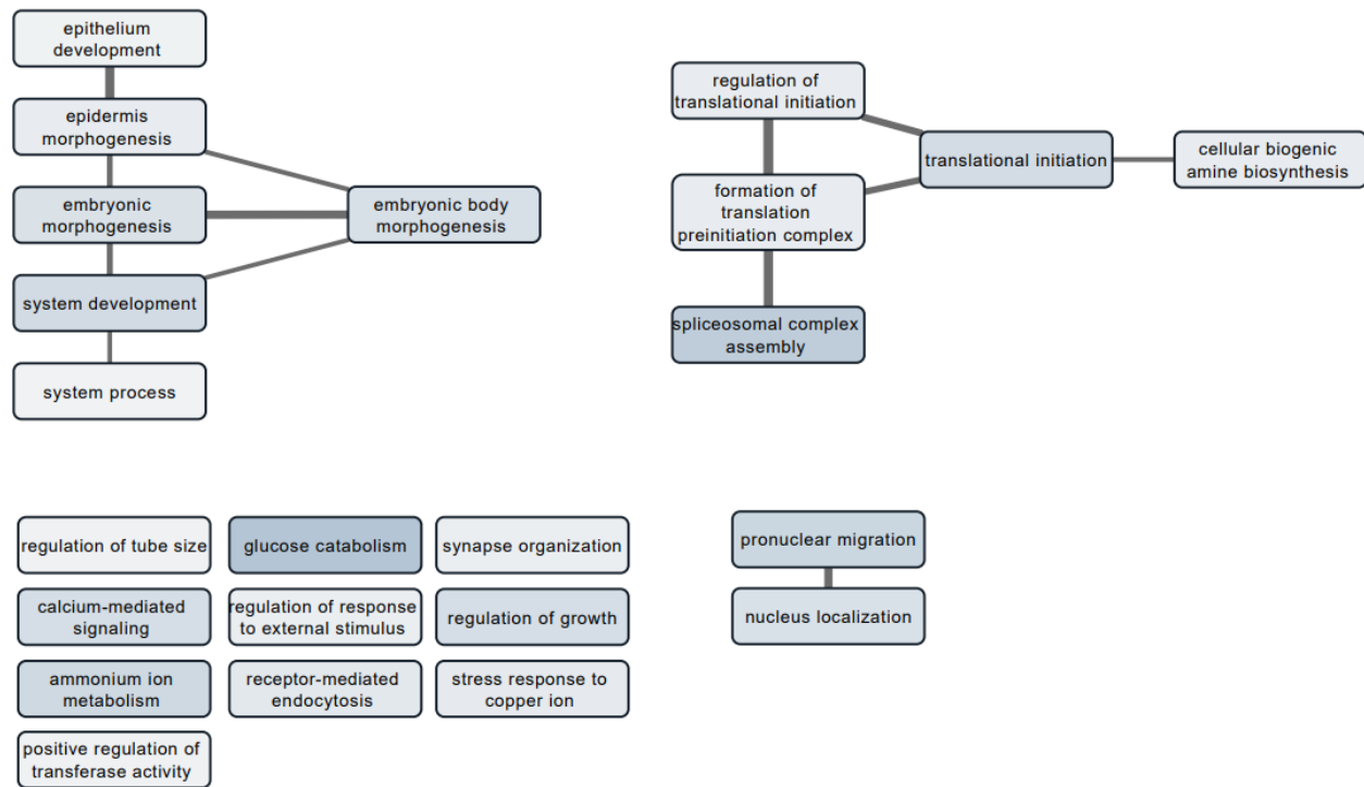
Supplementary Figure 7. Enriched GO term networks of biological processes for long term freezing.
