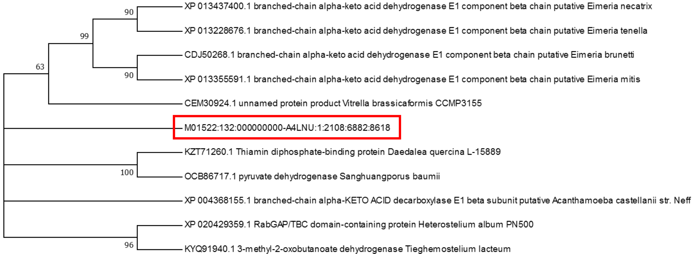
S9 Fig. Molecular Phylogenetic analysis by Maximum Likelihood method (BlastX homology search of M01522:132:000000000-A4LNU:1:2108:6882:8618). The evolutionary history was inferred by using the Maximum Likelihood method based on the Whelan And Goldman model. The bootstrap consensus tree inferred from 1000 replicates.
