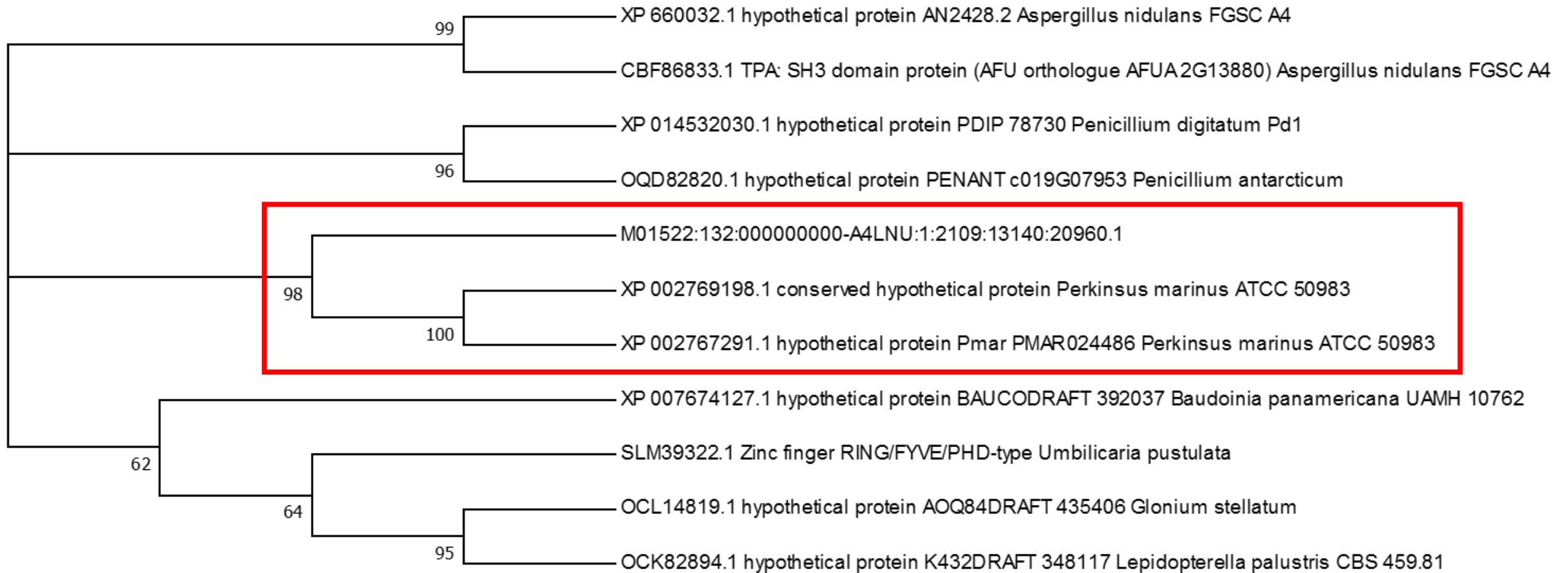
S8 Fig. Molecular Phylogenetic analysis by Maximum Likelihood method (BlastX homology search of M01522:132:000000000-A4LNU:1:2109:13140:20960.1). The evolutionary history was inferred by using the Maximum Likelihood method based on the Dayhoff matrix based model. The bootstrap consensus tree inferred from 1000 replicates.
