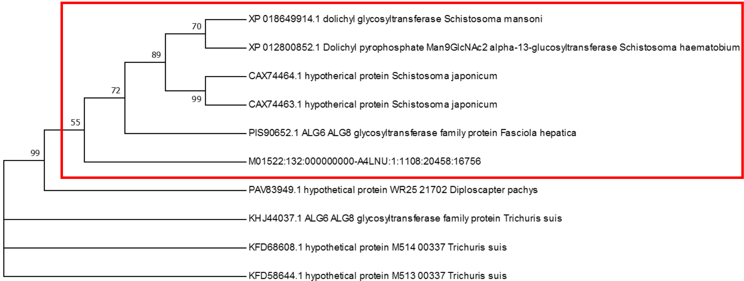
S3 Fig. Molecular Phylogenetic analysis by Maximum Likelihood method (BlastX homology search of M01522:132:000000000-A4LNU:1:1108:20458:16756). The evolutionary history was inferred by using the Maximum Likelihood method based on the Whelan and Goldman model. The bootstrap consensus tree inferred from 1000 replicates.
