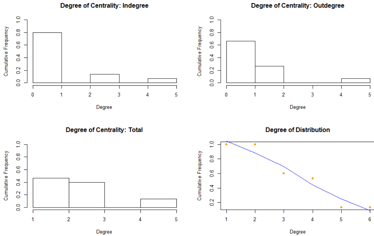
S1 Fig. Measuring connectivity with degree of centrality and distribution of the nodes in the network. Degree of centrality measures the amount of nodes connected to neighbor node, a node is important if it has many neighbors. X-axis represents the amount of connectivity (links) and y-axis represent the amount of nodes with said connectivity. Overall, the network has a few nodes that are highly connected representing a real network (power law).
