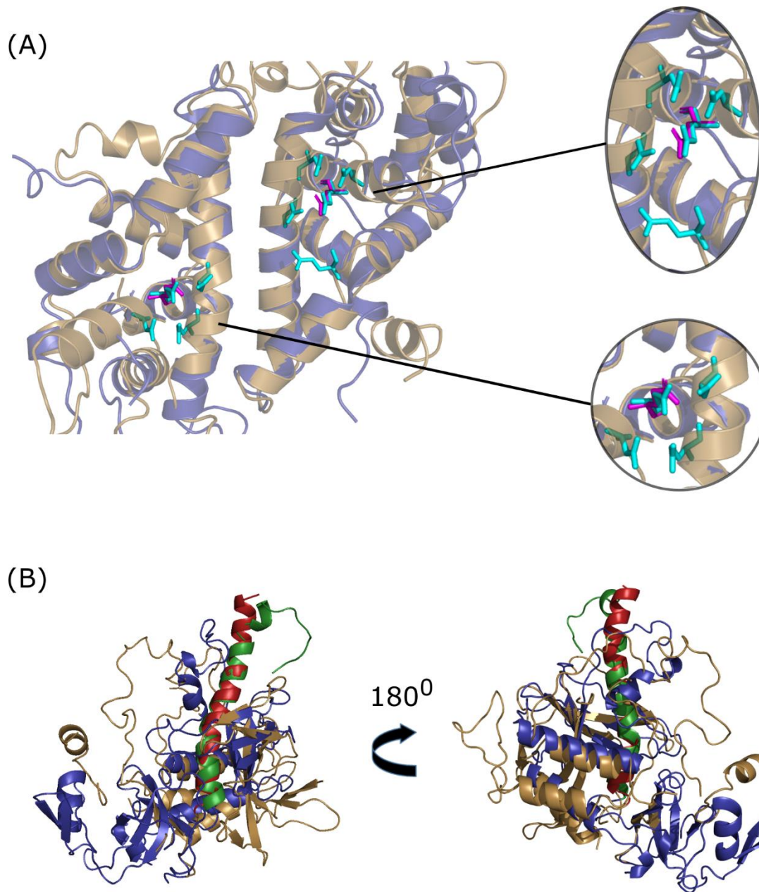
S1 Fig. Superimposition of Drosha and Dicer. (A) Superimposition of catalytic domains (RIIIda, RIIIdb) of Drosha and Dicer, together with the catalytic residues. Upper and lower insets at the right are of RIIIdb and RIIIda catalytic sites, respectively. (B) Back and front views of superimposition of CED domains (lower parts) of Drosha upon Dicer. Colors as the following: Drosha in sand, Dicer in deep blue, Catalytic residues in magenta (Drosha) or cyan (Dicer) sticks and Connector domains in firebrick (Drosha) or forest (Dicer).
