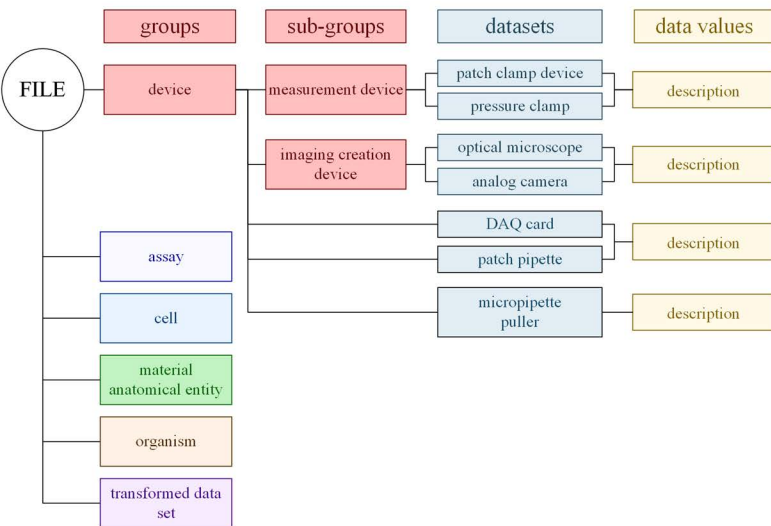
S2 Fig. (A) Directed root tree for the device arm showing the classes that describe the data. (B) Data architecture implemented to describe this arm with other main groups shown. The classes that were transformed into sub-groups, and datasets are denoted by pink and aqua.
