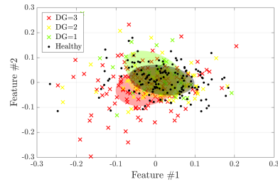
Figure 2: WDD analysis of the Messidor database. IsoMap features for the WDD analysis of the Messidor database with l = 0 and a = 1 .
