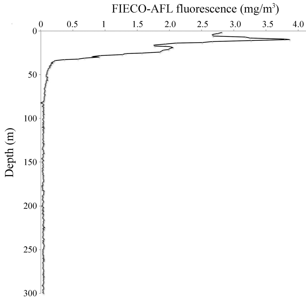
S2 Fig. FIECO-AFL for station 116, from surface to 300 m. The FIECO-AFL is an indirect measure of (chlorophyll) pigment concentration at different depths and indicates the abundance of photosynthetic microorganisms in the water column.
