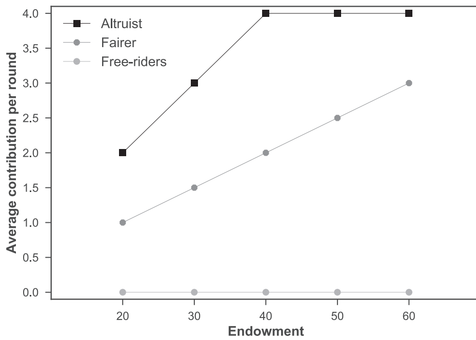
Fig S8: Ideal "pure" strategies based on our experiment design.
