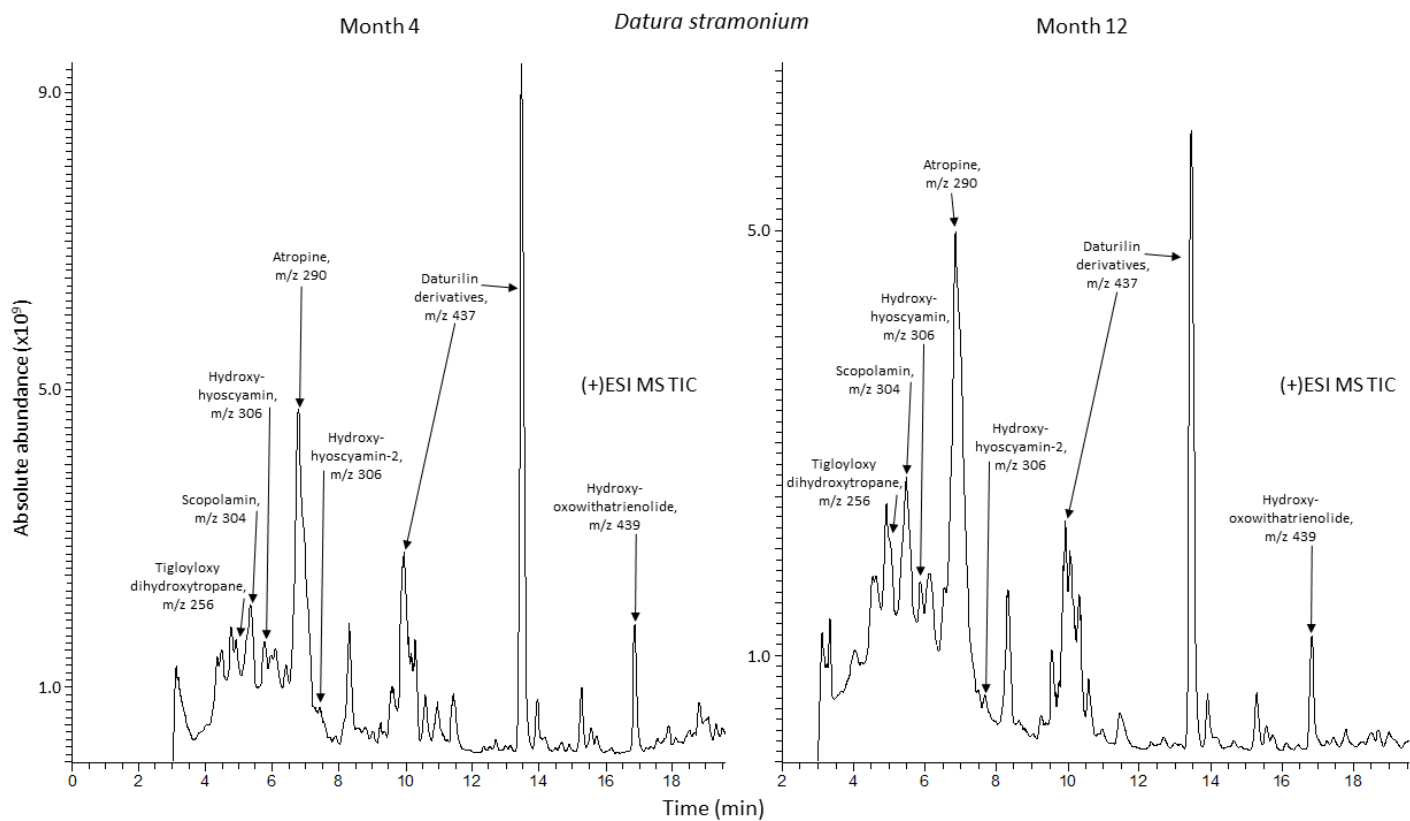
S2 Fig. Representative total ion current chromatograms (MS scanning mode from m/z 100 to m/z 1000) of eluates from Datura stramonium RAMES libraries after LCMS analyses following 4 and 12 month storage at -20^\circ\text{C} .
