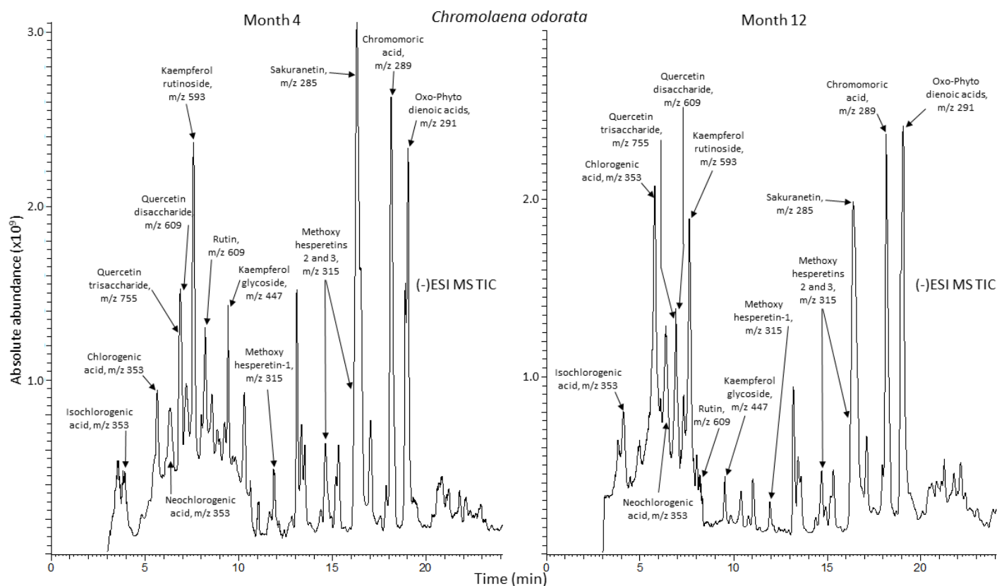
S1 Fig. Representative total ion current chromatograms (MS scanning mode from m/z 100 to m/z 1000) of eluates from Chromolaena odorata RAMES libraries after LCMS analyses following 4 and 12 month storage at -20°C.
