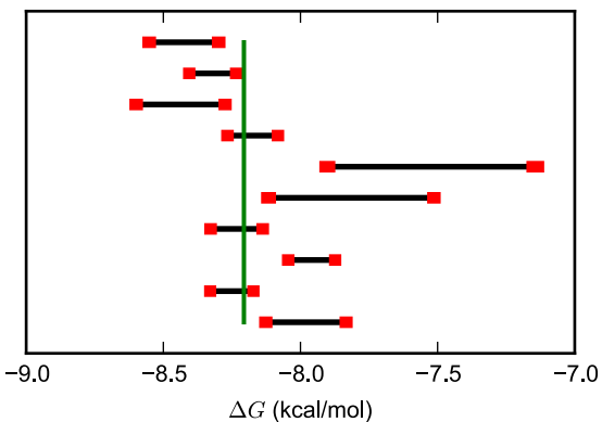
Bayesian approach
