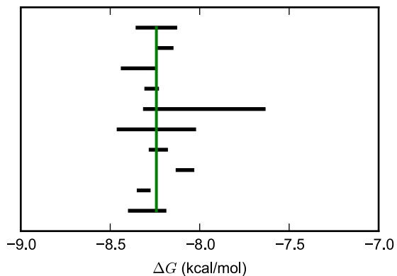
Nonlinear least squares
