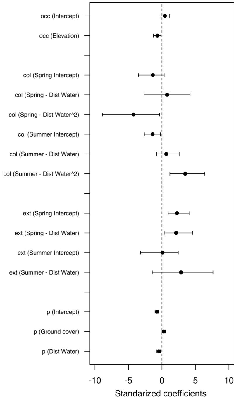
S2 Fig. Model coefficients and 95% credible intervals for the posterior distribution of the most parsimonious multi-season occupancy model for the American mink on Navarino Island for three seasons: summer and spring 2014, and summer 2015. Covariates include elevation, distance to water (marine coast and freshwater), and percentage of ground cover. Colonization and extinction parameters for Spring refer to the probability of colonization and extinction of sites from summer to spring. Colonization and extinction parameters for Summer refer to the probability of colonization and extinction of sites from spring to summer.
