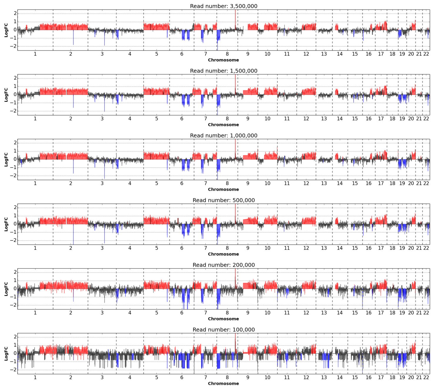
S18 Figure: Copy number profiles in cell line NCI-1650 cell #2 at 100 kbp resolution at different downsampling factors.
