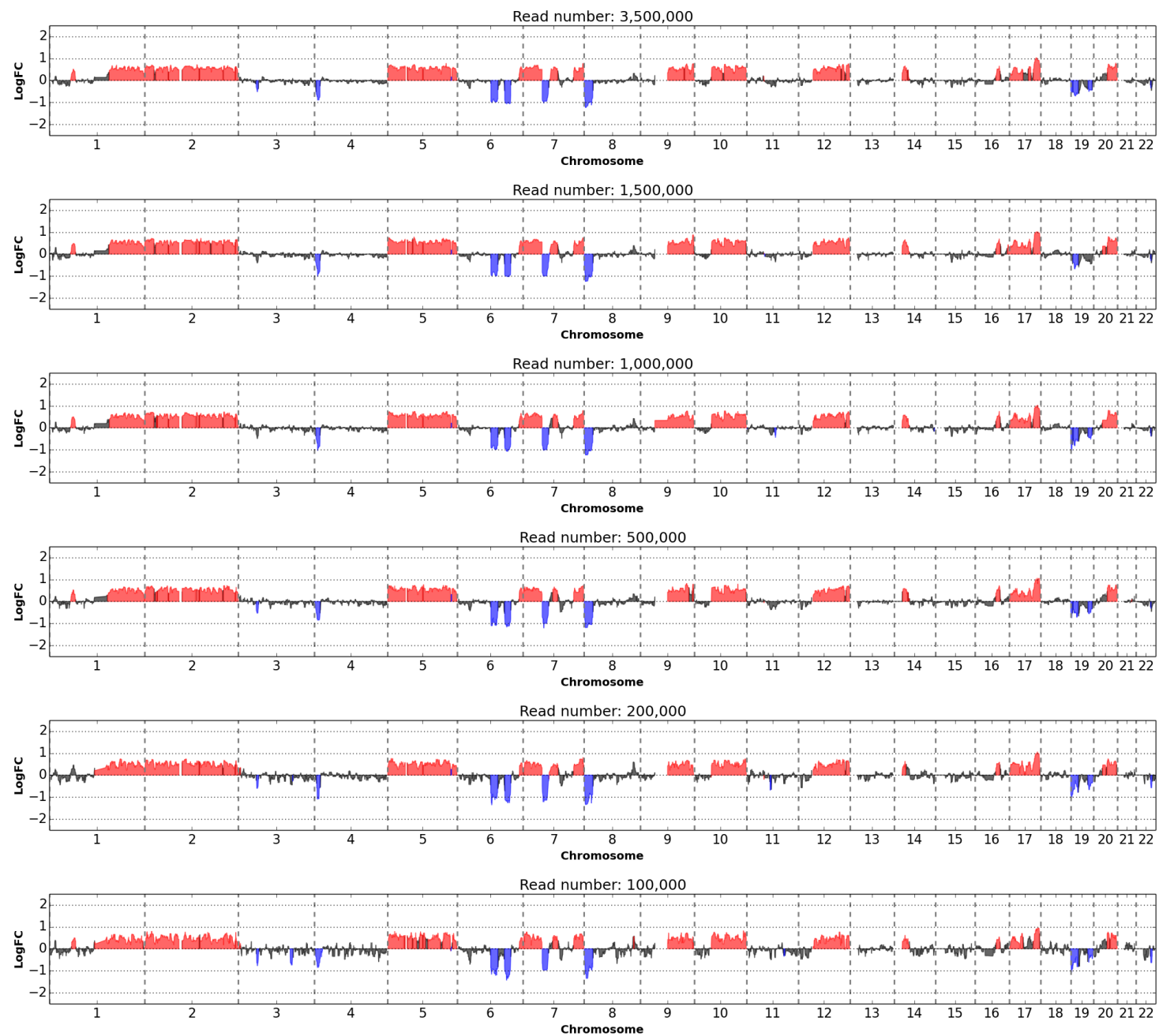
S13 Figure: Copy number profiles in cell line NCI-1650 cell #1 at 500 Kbp resolution at different downsampling factors.
