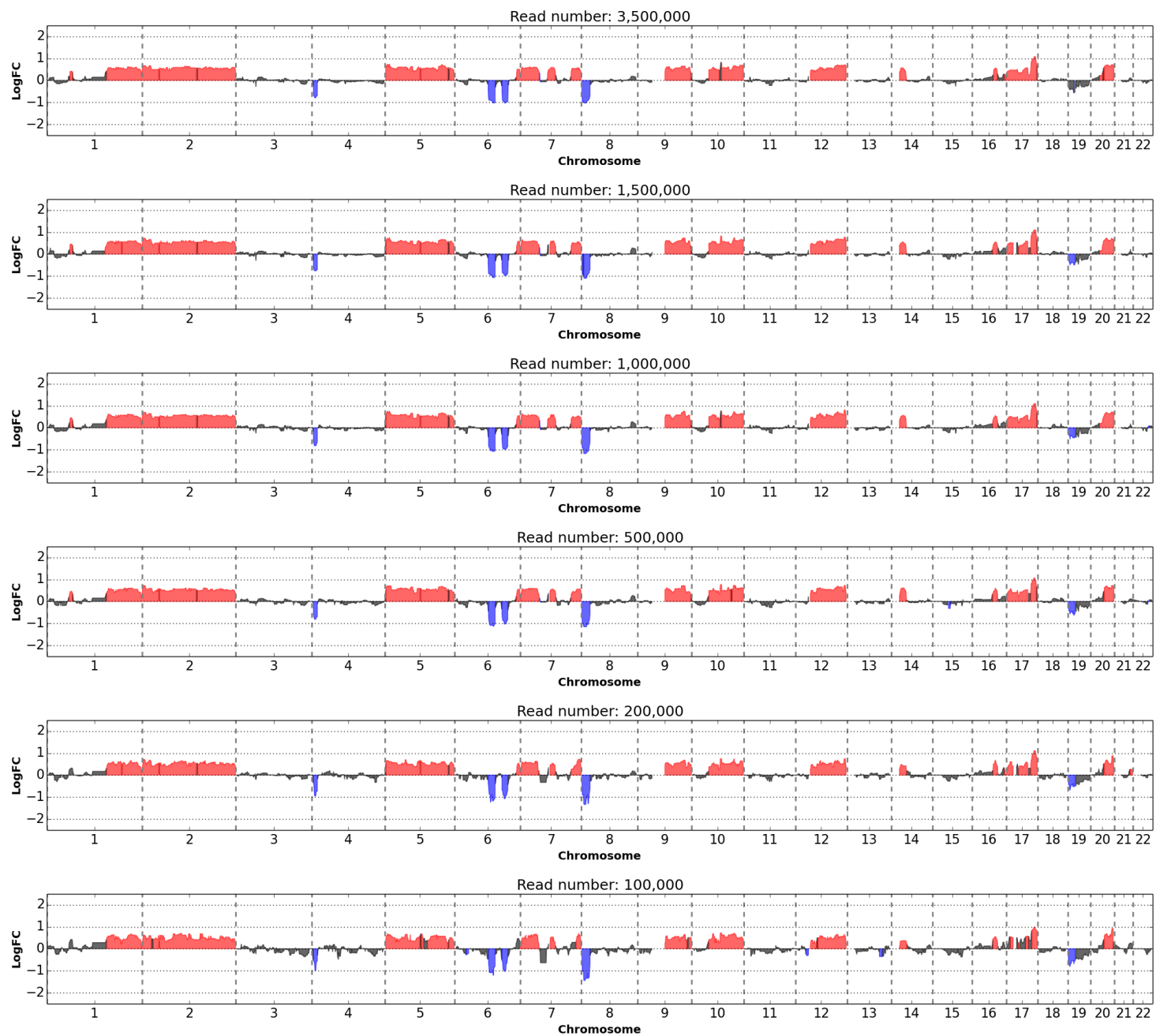
S12 Figure: Copy number profiles in cell line NCI-1650 cell #2 at 1 Mbp resolution at different downsampling factors.
