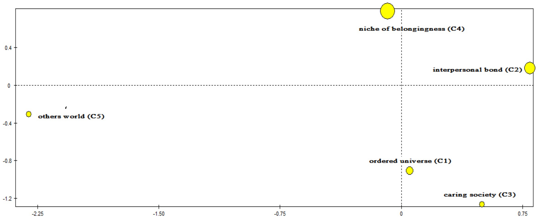
S1 Fig. Position of the symbolic universes on the MCA main factorial dimensions. Factor 1 vs. Factor 2
