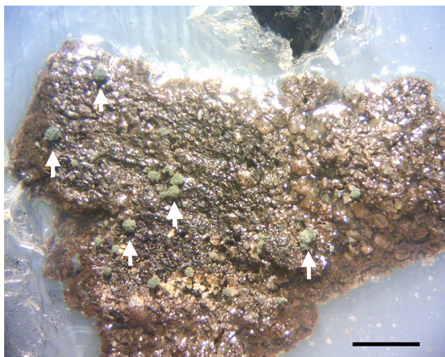
S2 Fig. Trichoderma harzianum TSTh20-1 (TSTh) sporulating (arrows) on bitumen after 7 d. The bitumen and the charcoal-TSTh inoculum (top) are pressed onto 2 % agarose. Bar represents 2 mm.
