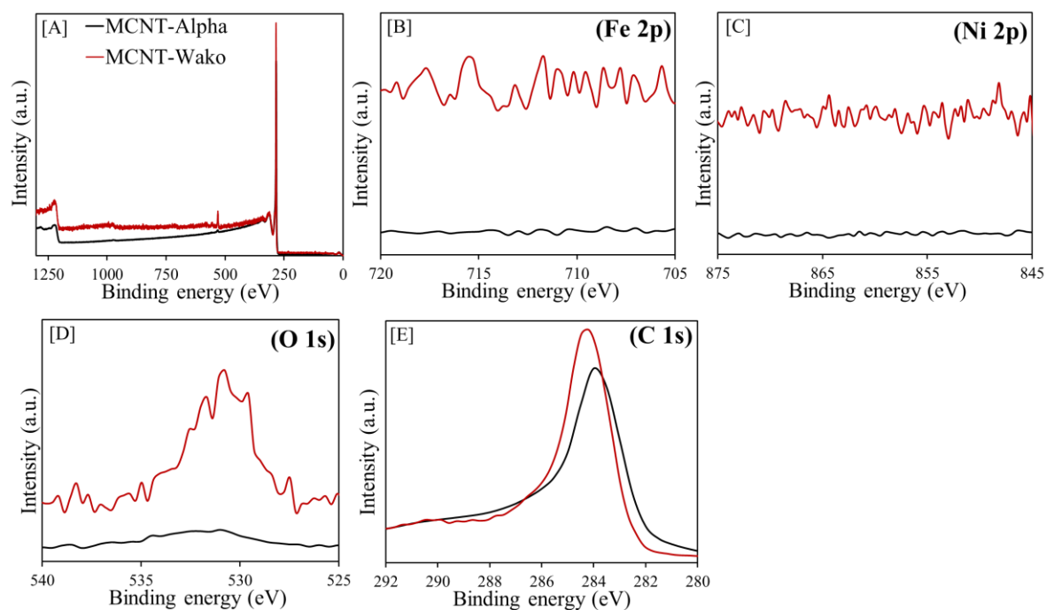
Fig. S2. [A] XPS scan for MCNT-Wako and MCNT-Alpha. Selected regions of high resolution scans for: [B] Fe 2p, [C] Ni 2p, [D] O 1s, and [E] C 1s spectra of MCNT-Wako and MCNT-Alpha. Only O 1s and C 1s peaks could be identified whereas, the Fe 2p and Ni 2p regions revealed only noise.
