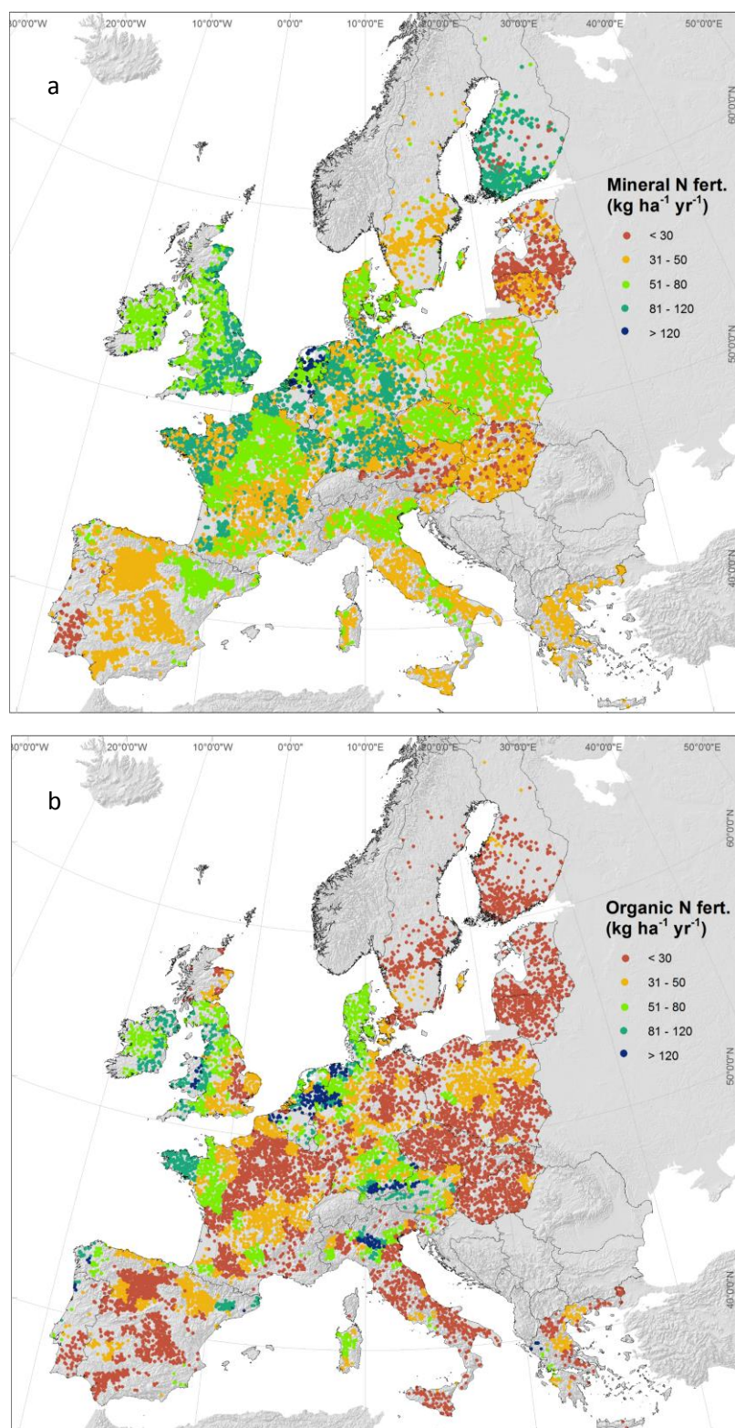
S1 Fig – Average (a) mineral and (b) organic N fertilization applied to LUCAS points. For the mineral fertilization, the values refer to the average N fertilization of the crop rotation since each crop (within the rotation) may have different rates based on agronomic requirement.
