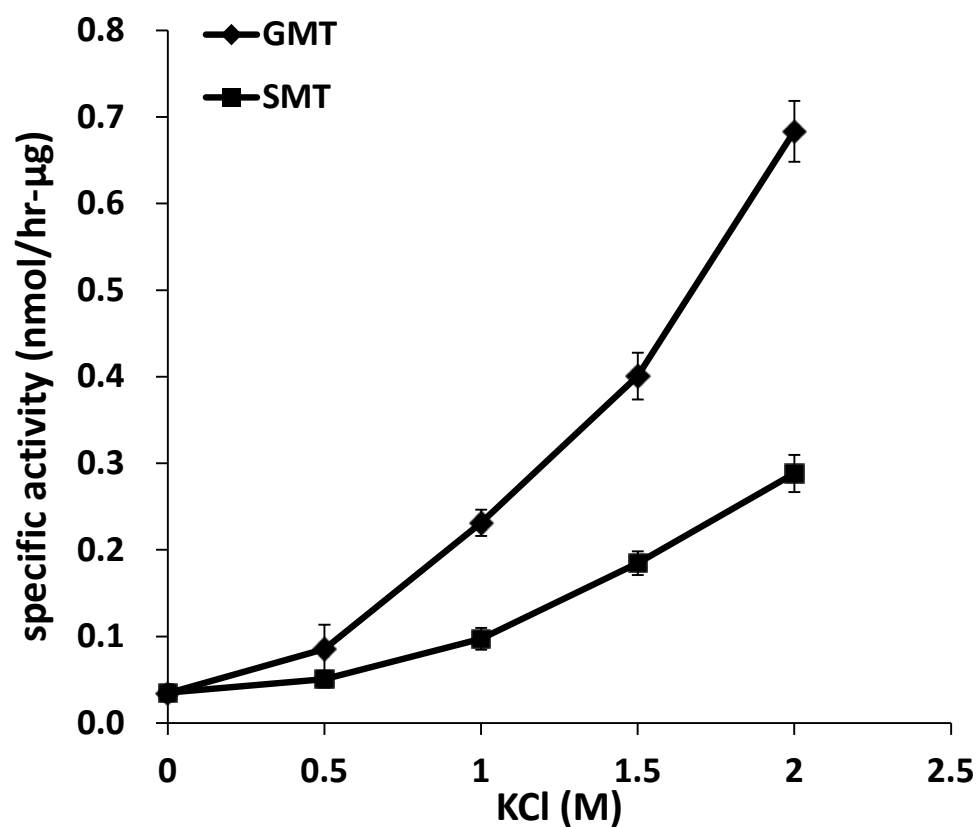
S1 Fig. rGSMT activities were promoted by potassium ions. Assay mixtures contained 0.1 M TES, pH 7.3, 1 mM SAM (containing 0.1 \mu Ci/2 pmol [ ^3 H-methyl]-SAM) and 0.5 M glycine or sarcosine under various concentrations of KCl. All the data points were averaged from independent triplicate experiments.
