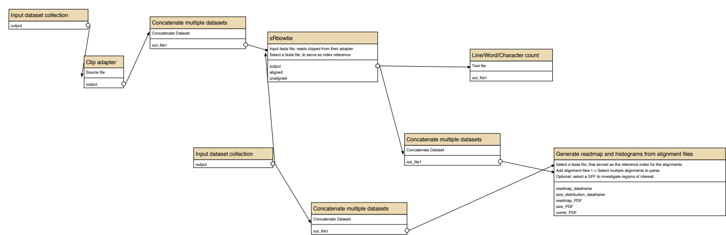
Metavisitor: Workflow for remapping in Use Cases 1-1,2,3
