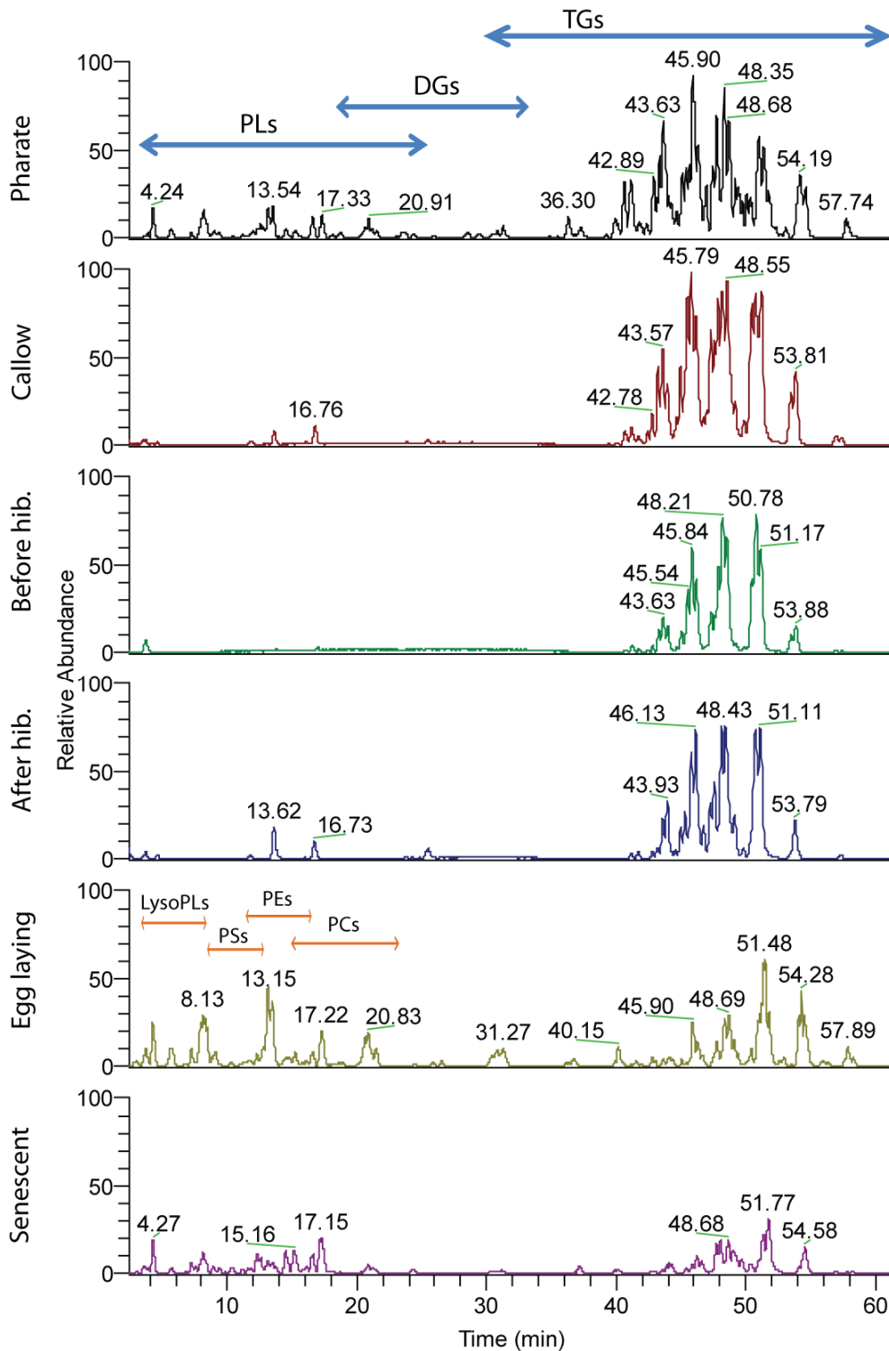
S4 Fig. Base peak chromatograms of total lipid extracts of fat bodies obtained from B. terrestris queens: pharate, callow, before hibernation, after hibernation, egg-laying, and senescent ones. Bidirectional arrows indicate the expansion of each type of lipid in chromatogram. Abbreviations: DG - diacylglycerols; LysoPL - lysophospholipides; PC – phosphatidylcholines PE - phosphatidylethanolamines; PL - phospholipids; PS - phosphatidylserines; TG- triacylglycerols.
