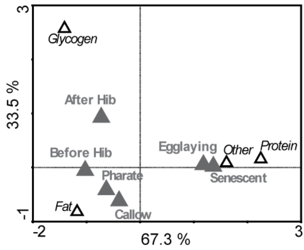
S3 Fig. Generated data visualization by CCA analysis shows the relationship between species (empty triangles) and samples (solid triangles).
