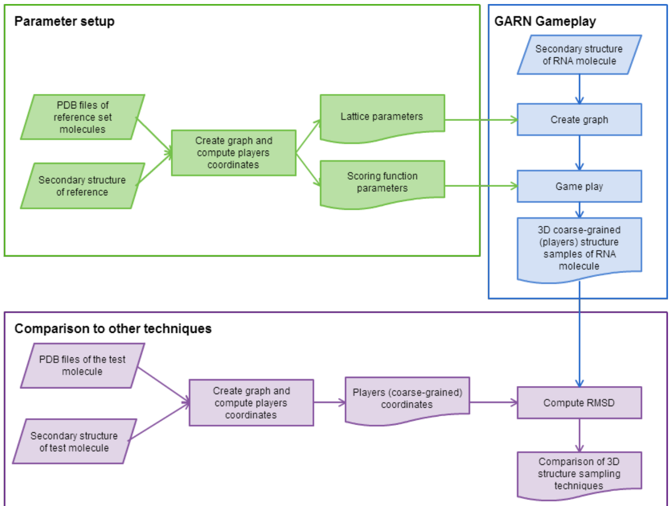
Figure S1: Overview. GARN has three parts: (i) the parameter setup for adjusting the game settings, (ii) the game process in GARN and (iii) comparisons with other published techniques.
