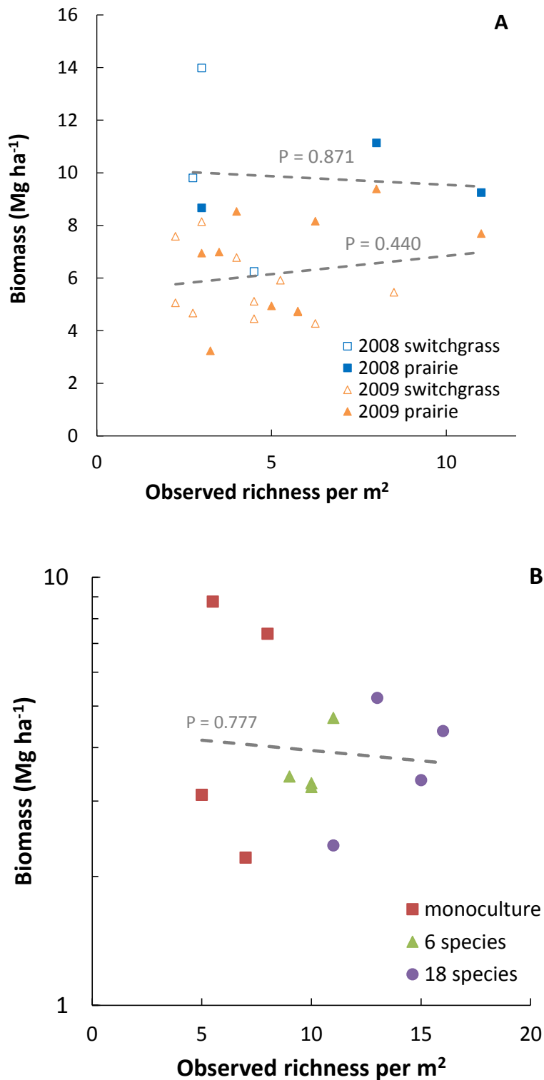
Figure S1. The relationship between average observed species richness and hand-collected biomass in the GLBRC field surveys (A) and the 2012 data from the LTER experiment (B). Please note the log scale in (B). P-values refer to the regression between observed species richness and biomass within a particular year.
