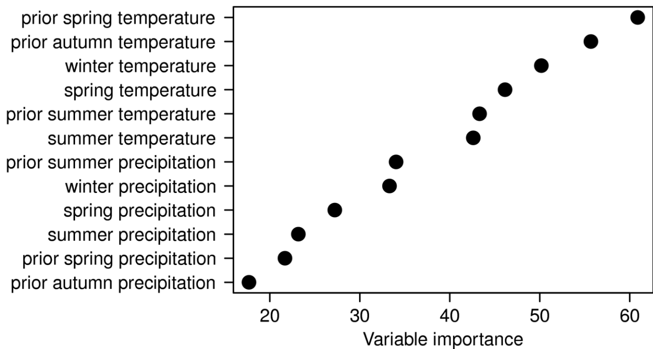
S3 Fig. Importance of climatic variables according to a 'random forest' analysis. Variable importance is given as the percental increase of the mean standard error under random permutation of the respective variables. See methods for the definition of seasons.
