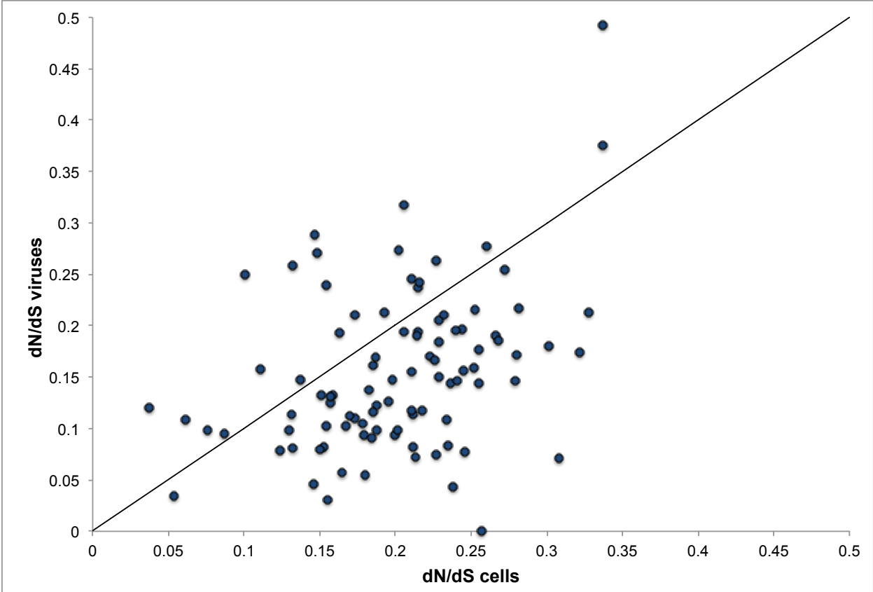
Figure S6. dN/dS for genes mapped by the viral metagenome versus dN/dS for the same genes mapped by the cellular metagenome. The line has a slope of 1.
