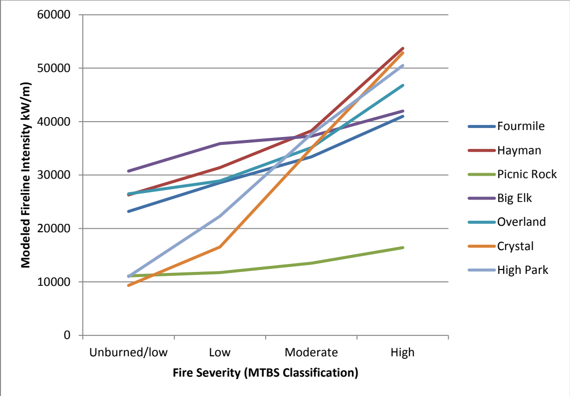
Figure S1. MTBS fire severity classification (observed) and median fire line intensity (modeled). The comparison was used as a measure of verification of the modeled fire behavior.
