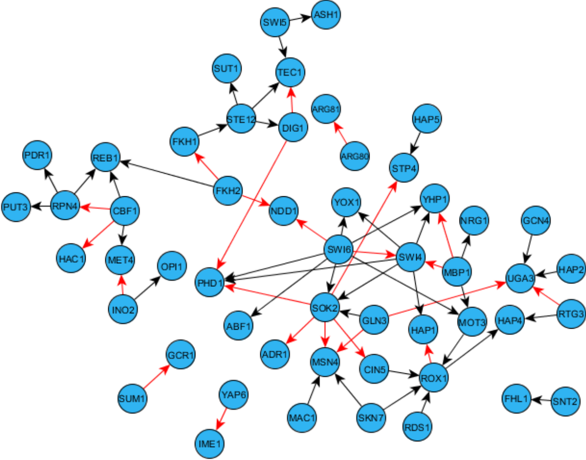
Figure S2: Direct regulatory interactions between transcription factors in gold-standard gene regulatory network #2. Inhibiting edges are shown with red, and excitatory edges are shown with black.
