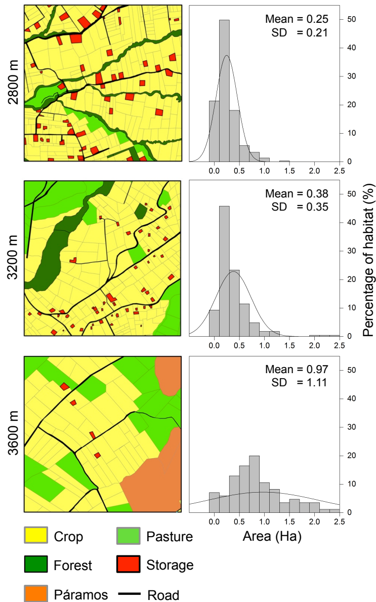
606 Figure S1: Habitat mapping of the three studied 1-km 2 grid cells at their respective elevations 607 (2800, 3200 and 3600 m) and the corresponding frequency distribution histograms of field 608 areas.
