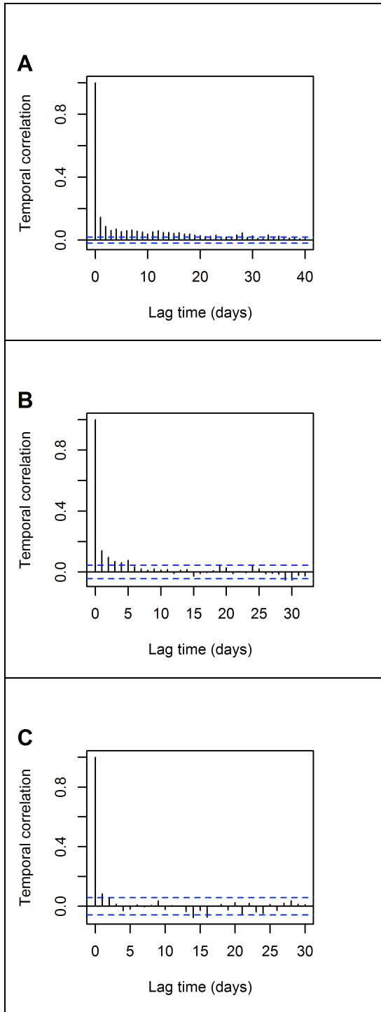
Figure S2. Correlation in residuals ordered in time with lag time in days for the overall trend models including seasonality using landings in (A) principal green turtle, Chelonia mydas , fishing communities, (B) commercial center for the Awastara community, and (C) communities using the Refugio de Vida Silvestre Cayos Perlas fishing area.
