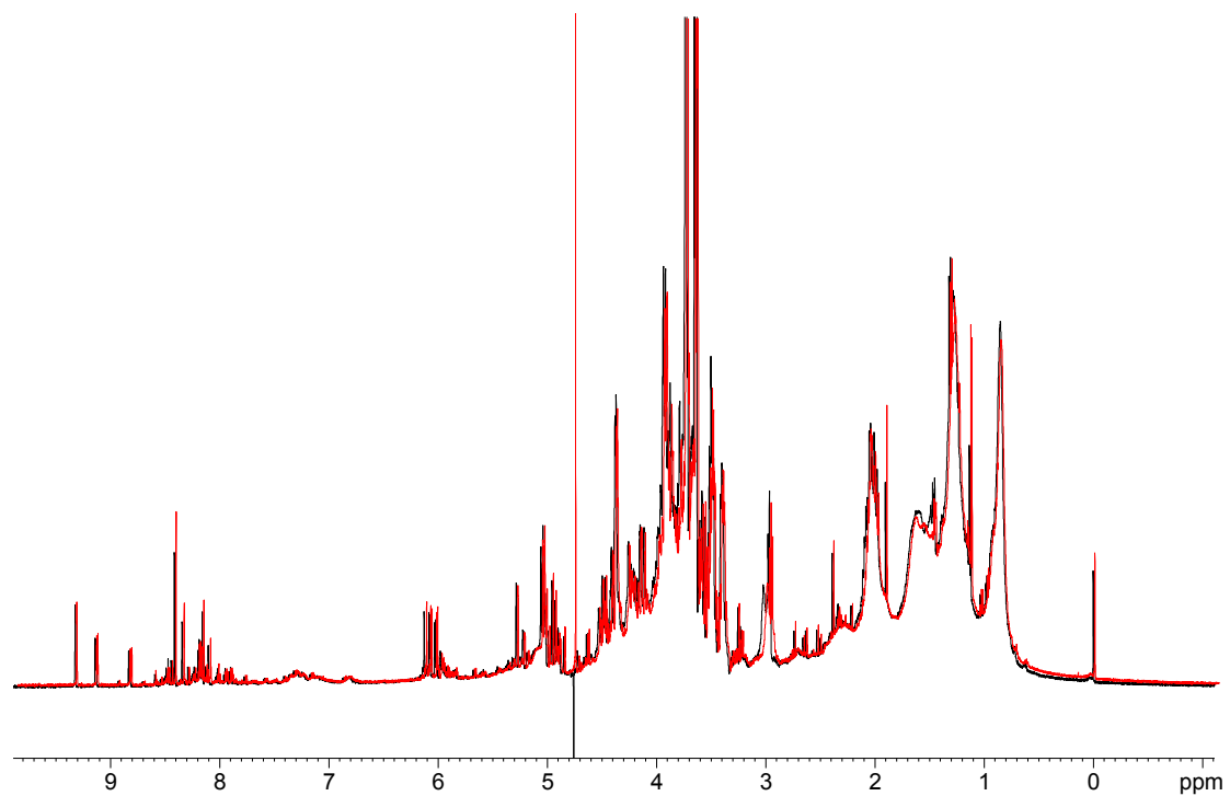
Figure S1. ^1\text{H} NMR spectra of the extracted intracellular polar metabolites from wild-type Clostridium thermocellum before (black) and after (red) quenching experiments.
