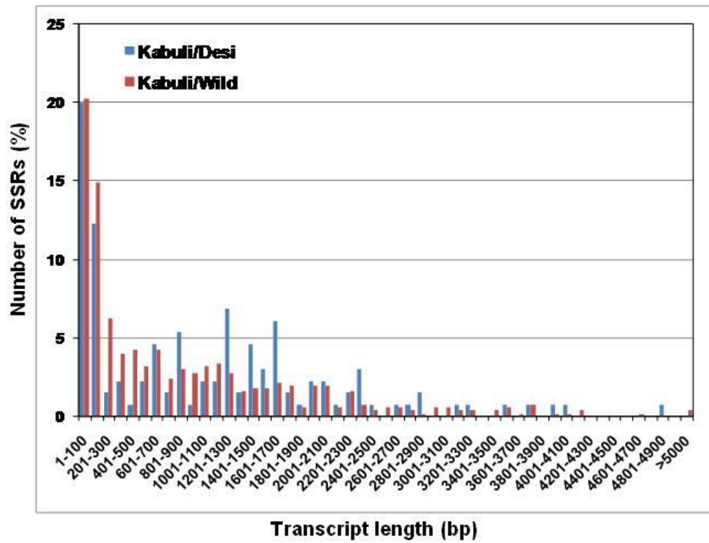
Figure S6. Distribution of polymorphic SSRs between kabuli/desi and kabuli/wild chickpea along the transcript length.
