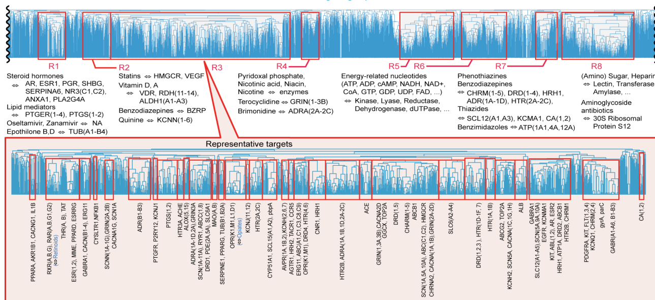
Figure S2: Hierarchical clustering on drug-target pairs where R1 to R8 are specified with brief descriptions on representative drug-target pairs or targets.
