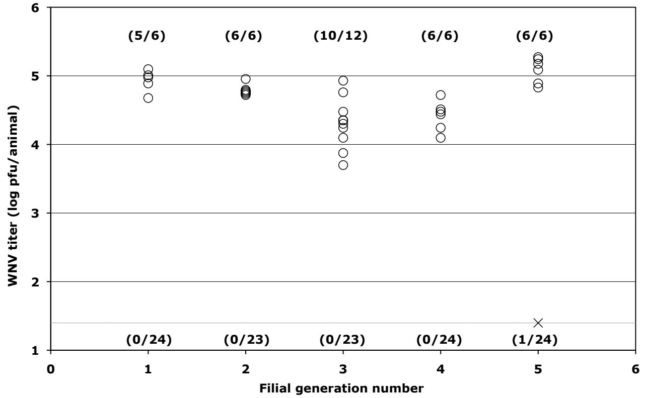
Figure S3. The WNV resistance phenotype observed in Ago2 414 flies is caused by a maternal cytoplasmic factor.
