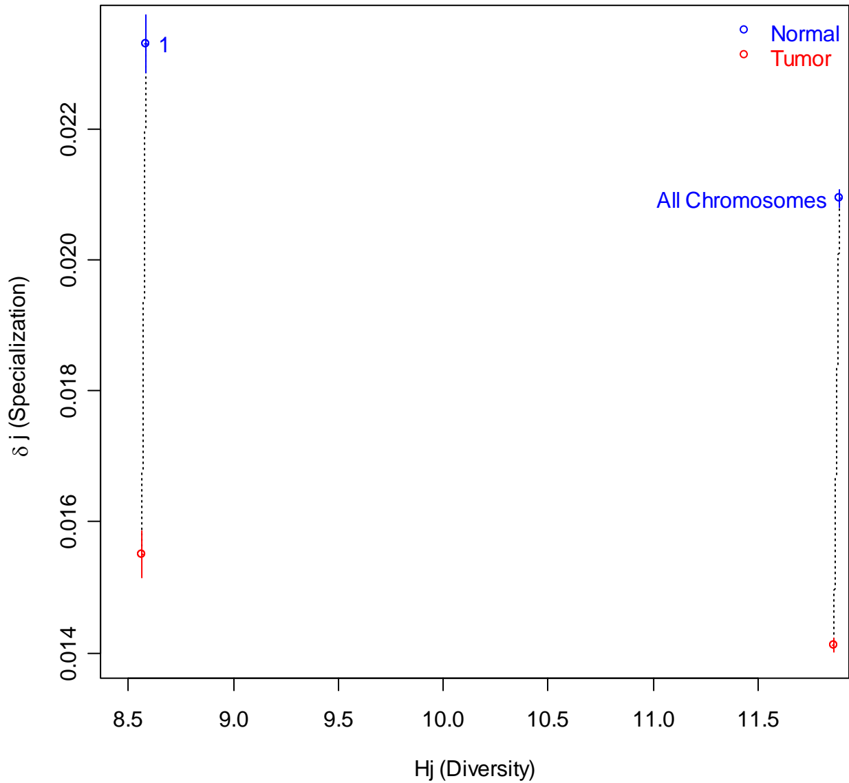
Fig. S10. Estimated values of H_j (diversity) and \delta_j (specialization) in chromosomes 1 and the set of all chromosomes taken together. Dataset C . Open circles are plotted in the mean of the 2000 bootstrap replicates for each parameter and the corresponding approximate 95% confidence intervals are plotted as continuous lines in each axis. This figure amplifies grey box of Fig. 2.
