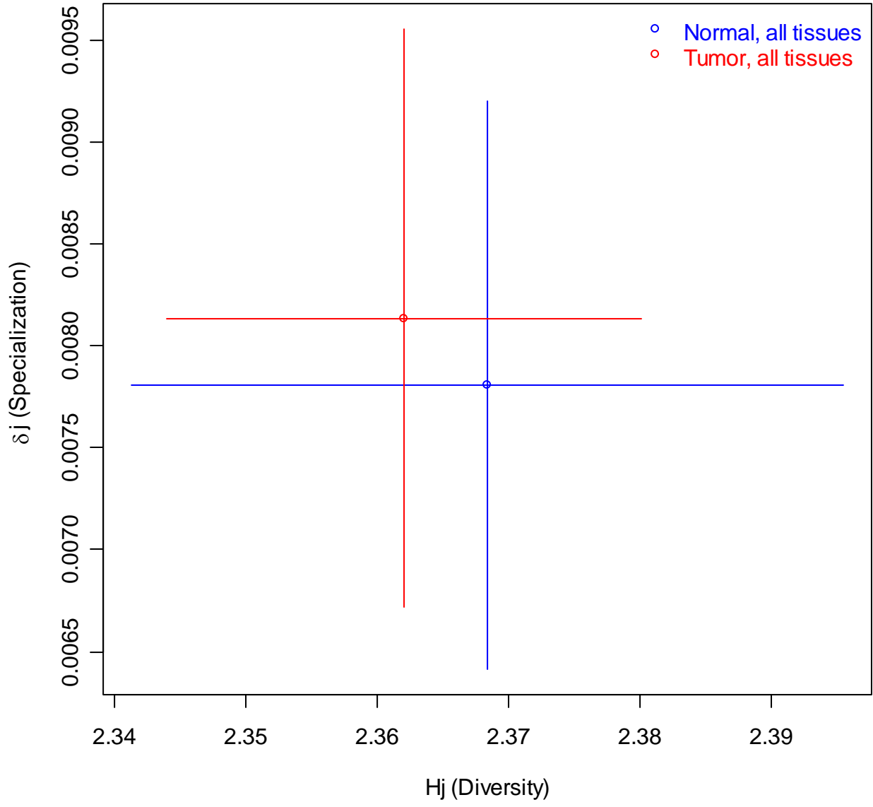
Fig. S7. Estimated values of H_j (diversity) and \delta_j (specialization) in the chromosome Y (dataset C, HTM). Open circles are plotted in the mean of the 2000 bootstrap replicates for each parameter and the corresponding approximate 95% confidence intervals are plotted as continuous lines in each axis. This figure amplifies the green box of Fig. 2.
