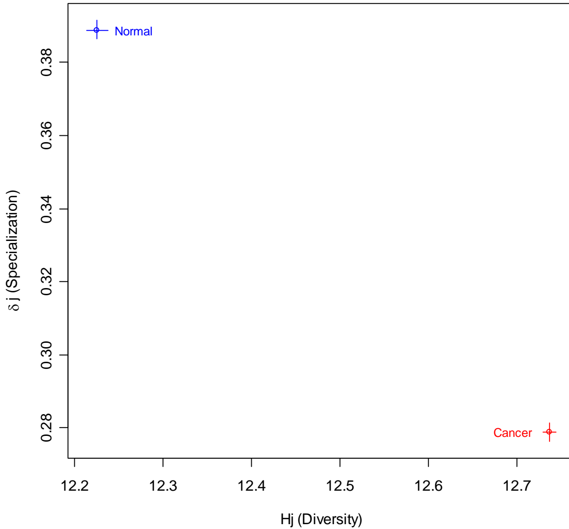
Fig. S6. Estimated values of H_j (diversity) and \delta_j (specialization) in normal and cancerous transcriptomes obtained by grouping all organs in dataset B (mouse data). Open circles are plotted in the mean of the 2000 bootstrap replicates for each parameter and the corresponding approximate 95% confidence intervals are plotted as continuous lines in each axe.
