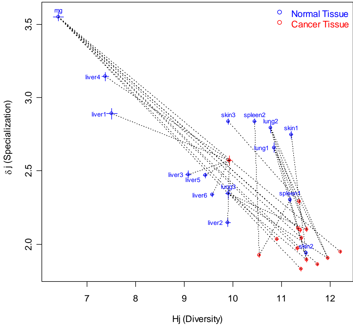
Fig. S4. Estimated values of H_j (diversity) and \delta_j (specialization) in each one of the libraries of dataset B (mouse data), non-grouped analysis. Open circles are plotted in the mean of the 2000 bootstrap replicates for each parameter and the corresponding approximate 95% confidence intervals are plotted as continuous lines in each axis. Discontinuous lines join comparable libraries (same tissue). For clarity the graph for each set of comparable mouse libraries are presented in Fig. S5.
