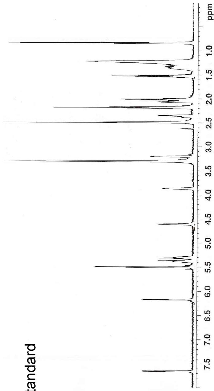
(B) HPLC fraction 2 from P. homomalla
