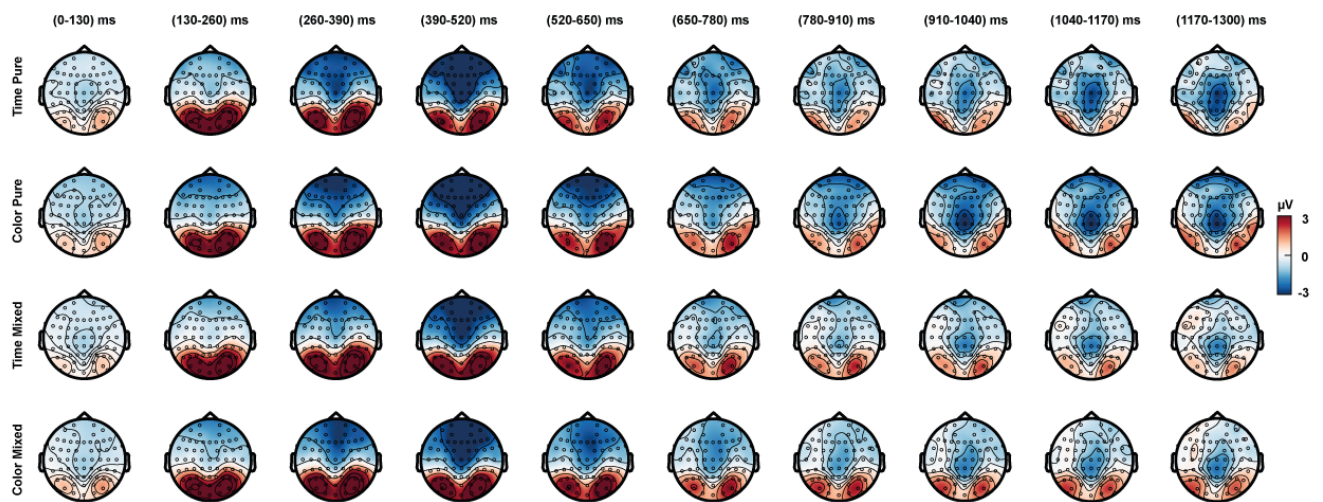
Fig S2. Topographies by task at S1 Onset. Mean topographies of the EEG signal in 130 ms windows during S1 onset for trials longer than 1300ms. Each row represents a different task condition.
