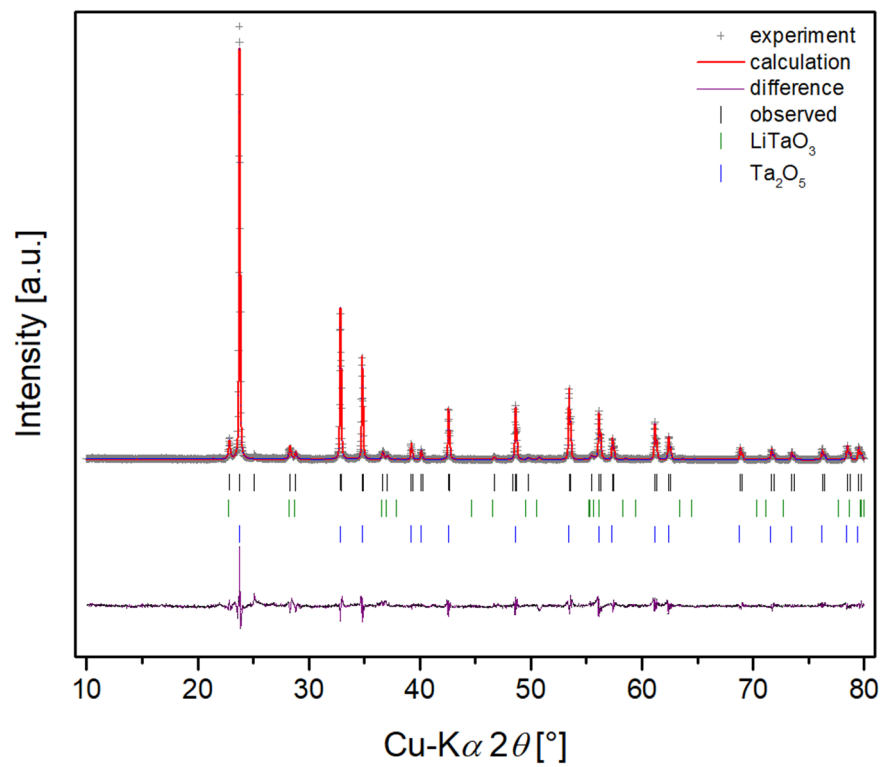
Figure S1. XRD diffraction Rietveld refinement results of \text{LiTaO}_3 powder with 11% \text{Ta}_2\text{O}_5 content.
