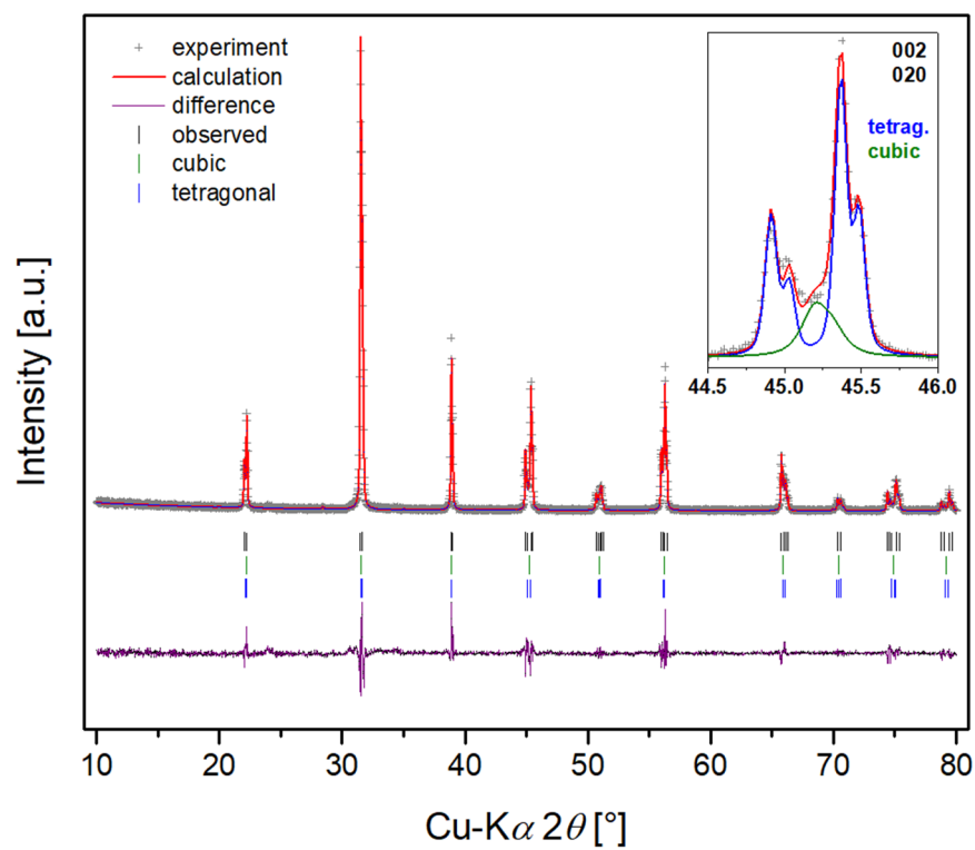
Figure S1. XRD diffraction Rietveld refinement results of BaTiO 3 powder. Inset shows composition of 002/020 reflection with respect to cubic and tetragonal fraction.
