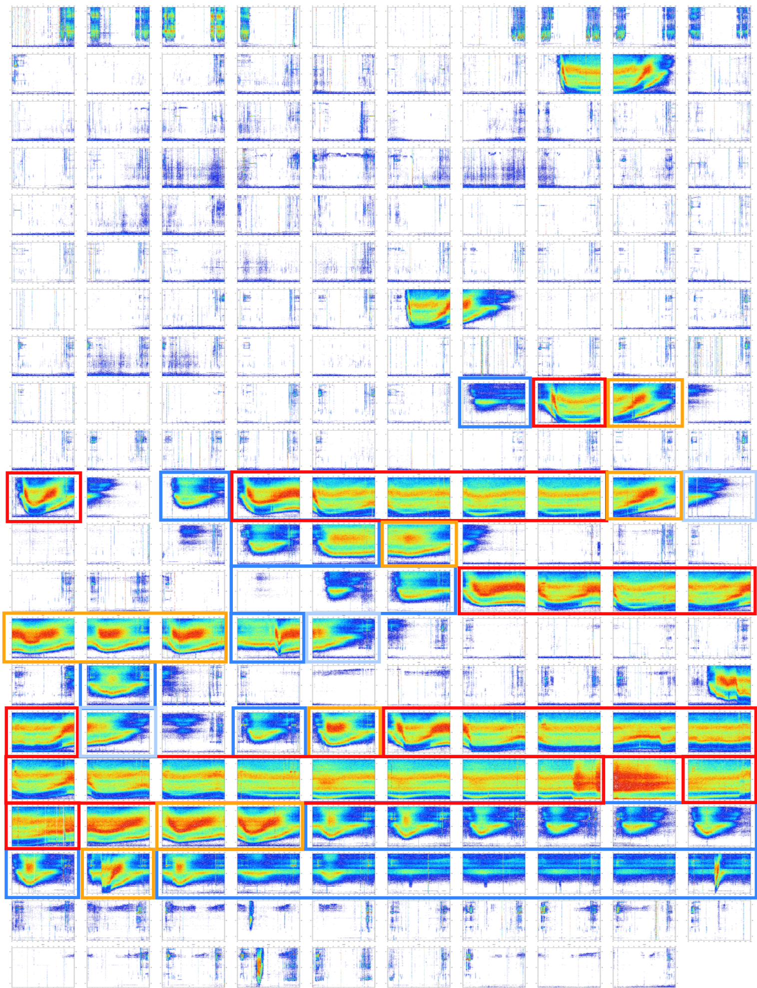
Supplemental Figure S3: Daily spectrograms for year 2013 (Julian days 1-200). Each spectrogram begins at 12:00 UTC and end at the same hour the next day. Frequency range: 1.5 - 6.5 Hz. Color boxes show the results from the hierarchical classification (see Fig 8).
